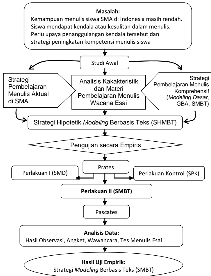
Gambar 2. Alur Penelitian
