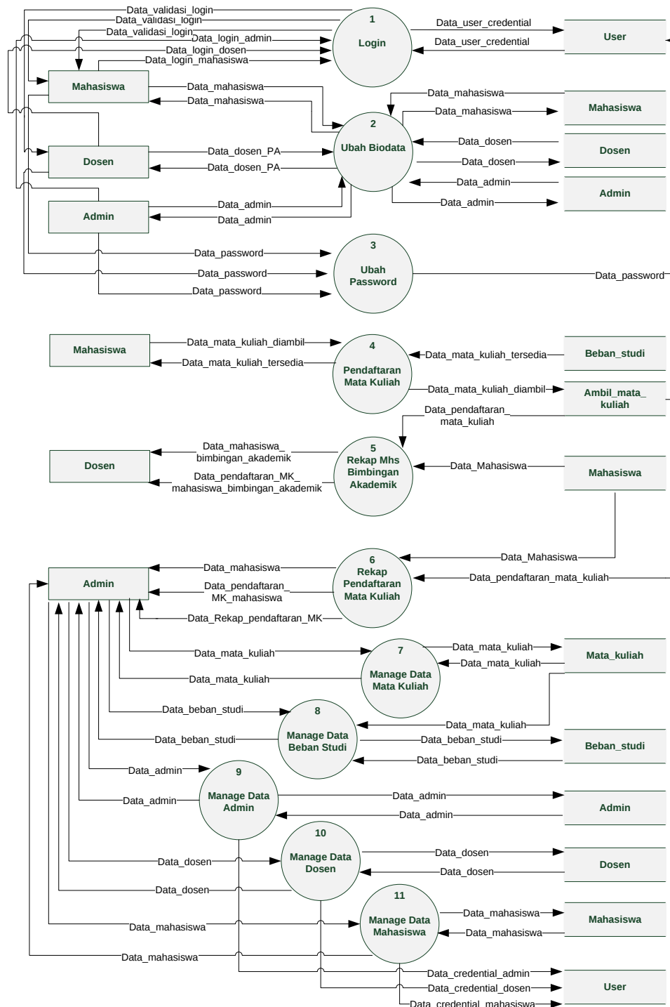
Gambar 3. DFD level 1
