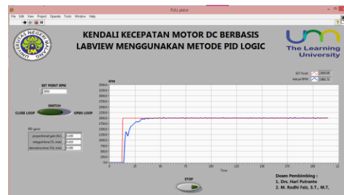
Gambar 17. Data 2000 RPM
