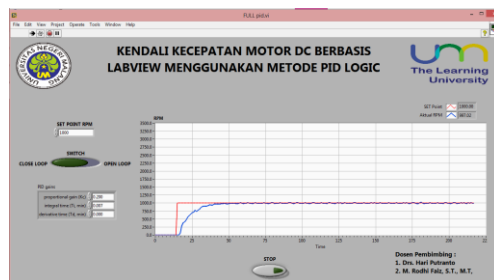
Gambar 19. Data 1000 RPM
