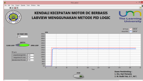
Gambar 14. Data 2000 RPM
