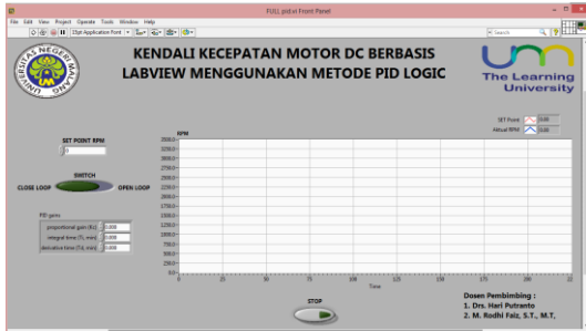
Gambar 7. Front Panel
