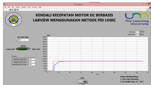
Gambar 16. Data 1000 RPM
