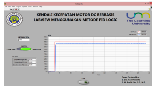
Gambar 15. Data 3000 RPM
